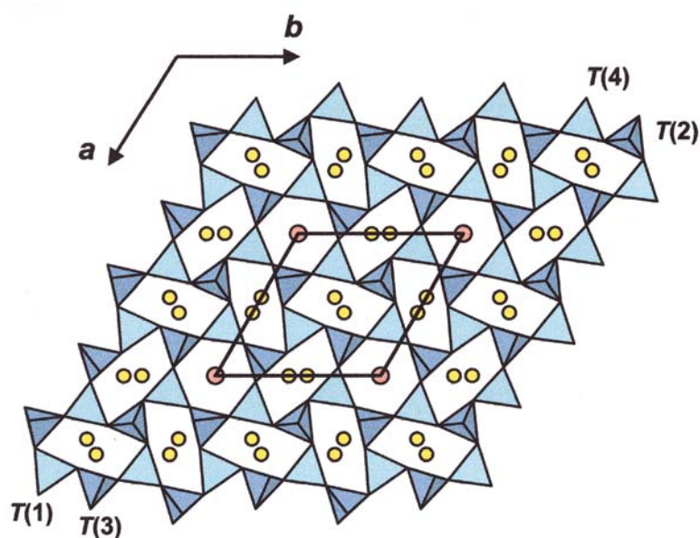
FIG. 1. The crystal structure of the nepheline projected onto (001). The T(2) and T(3) tetrahedra ( \text{Si} > \text{Al} ) are navy blue, the T(1) and T(4) tetrahedra ( \text{Al} > \text{Si} ) are greenish blue, the K sites are shown as orange spheres, and the Na sites, as yellow spheres.
